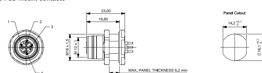
Back Mount with M16 x 1,5 mounting thread and PCB mount contacts
